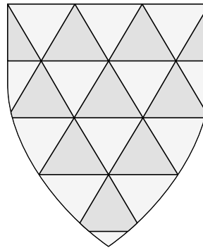
Masculy (2)
