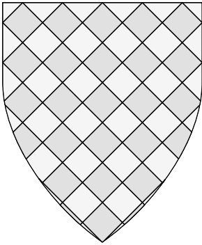
Lozengy Bendwise (2)
